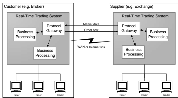
Figure 1: Integration between real-time trading systems
