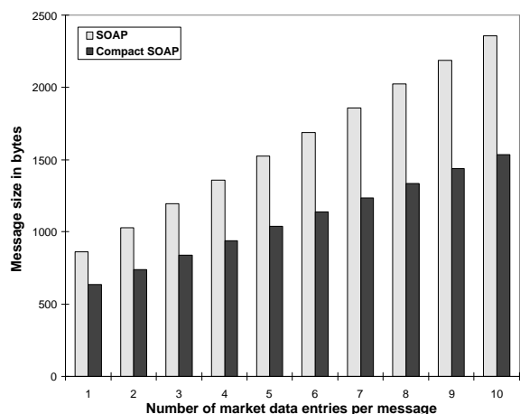
Figure 15: Message size reduction when compact XML tags are used
