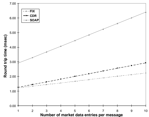
Figure 8: Round-trip times over 10 Mbps network
