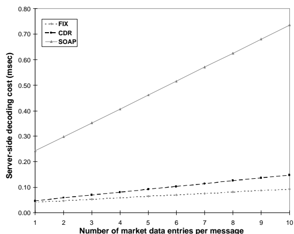
Figure 11: Server-side decoding costs
