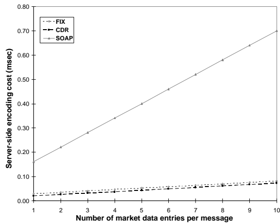
Figure 10: Server-side encoding costs
