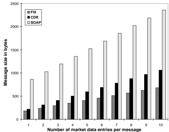
Figure 4: Message size comparison of the wire formats
