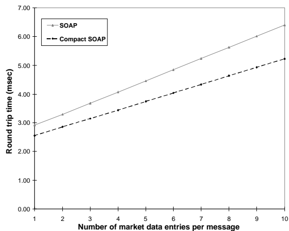
Figure 16: Round-trip times for compact SOAP messages over 10 Mbps network
