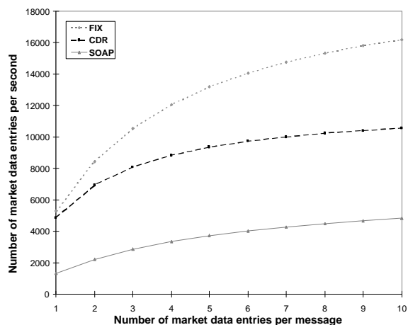
Figure 12: Throughput over 10 Mbps network
