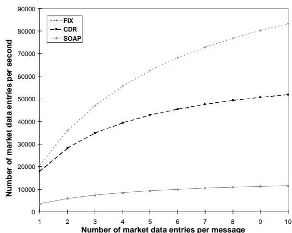
Figure 13: Throughput over 100 Mbps network
