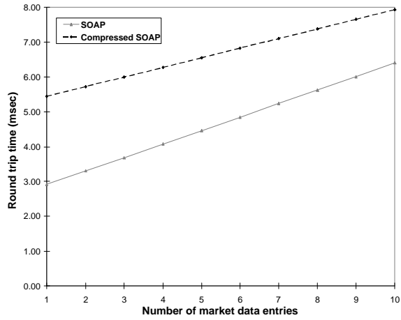
Figure 14: Round-trip times over 10 Mbps network for compressed and uncompressed SOAP messages
