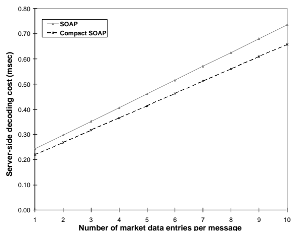
Figure 17: Decoding costs for compact SOAP messages
